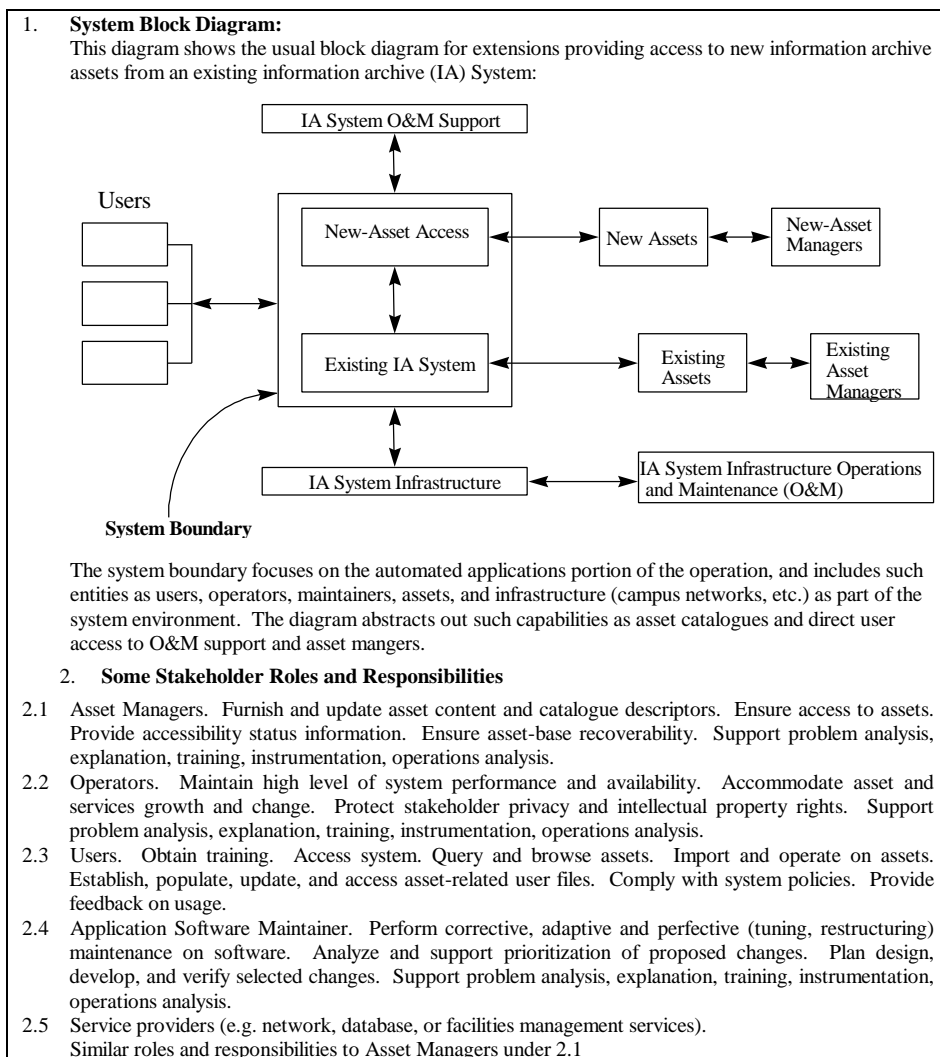
Figure 4. Information Archive Extension Domain Model
