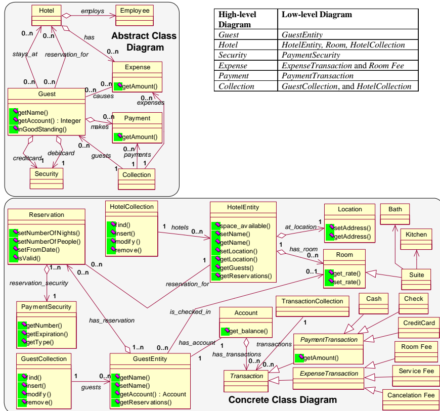
Figure 2. High-level and low-level class diagrams of HMS and mapping table
