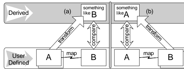
Figure 1. View transformation and mapping to complement view comparison
