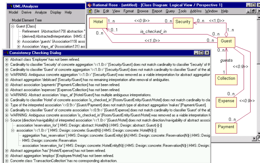
Figure 5. UML/Analyzer tool depicting inconsistencies
